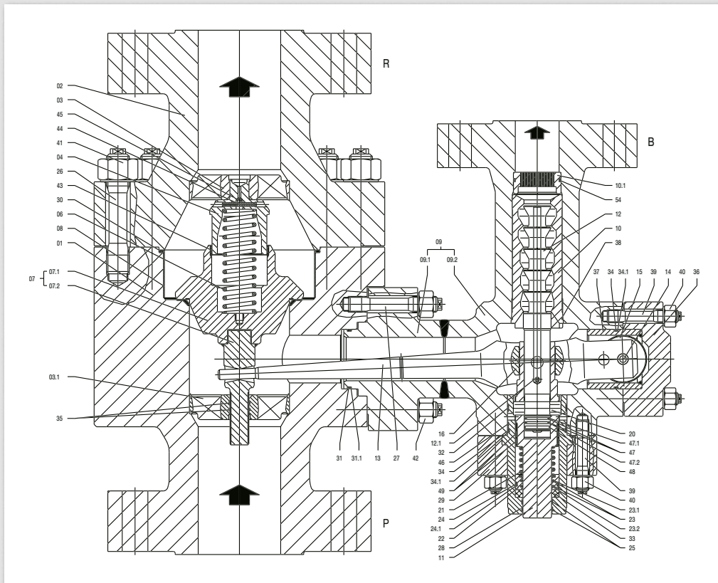
Fig 1: Valve type MRM
